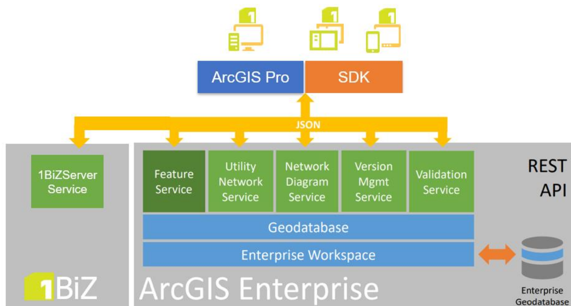
Figure 1 : Architecture générale
