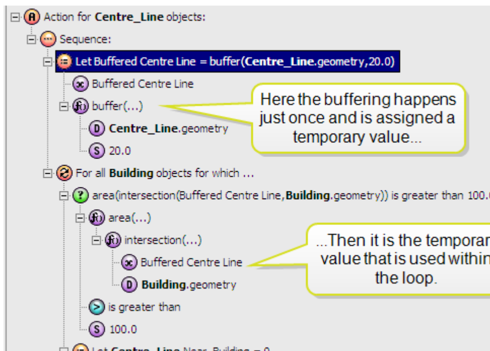
Figure 1-8: Buffer is calculated only once
